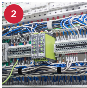
2 Building Automation System Cabinet
